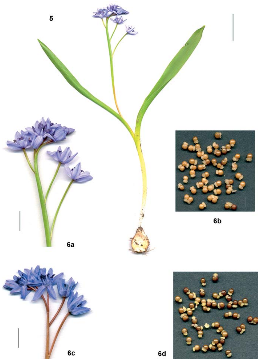
Figs 5–6. 5 – Scilla bifolia subsp. bifolia var. bohemica : general habit, live plant of the holotype specimen (locality: central Bohemia, Kobylnice village near Kolín), scale bar = 3 cm. 6 – a, b: Scilla bifolia subsp. bifolia var. bohemica (locality: central Bohemia, Kobylnice village near Kolín): a – inflorescence, live plant of the holotype specimen, scale bar = 1 cm, b – seeds, scale bar = 5 mm; c, d – S. bifolia subsp. bifolia var. drunensis : c – inflorescence, live plant (locality: central Moravia, Náměšť na Hané village near Olomouc), scale bar = 1 cm, d – seeds (locality: South Moravia, Moravské Bránice village near Ivančice), scale bar = 5 mm.
